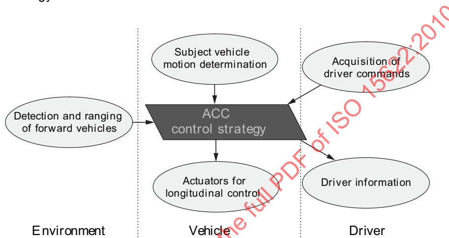
Figure 1 — Functional ACC elements
