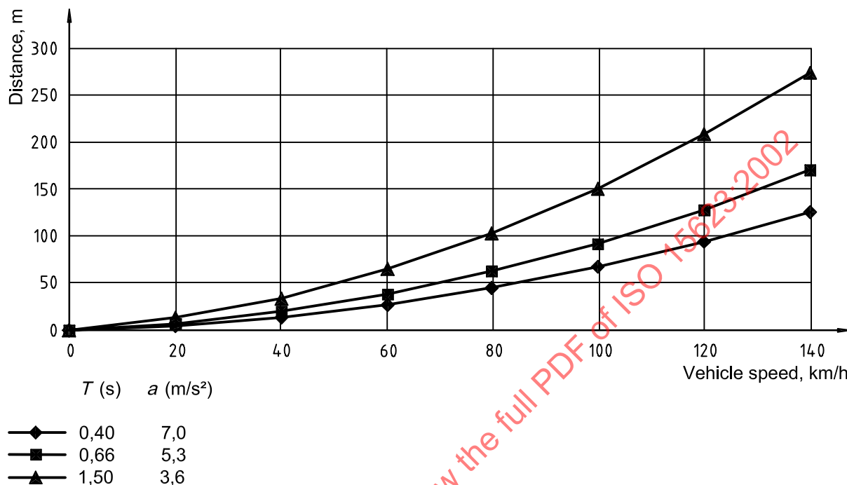
Figure A.5 — Relationship between vehicle speed and stopping distance for stationary obstacle
