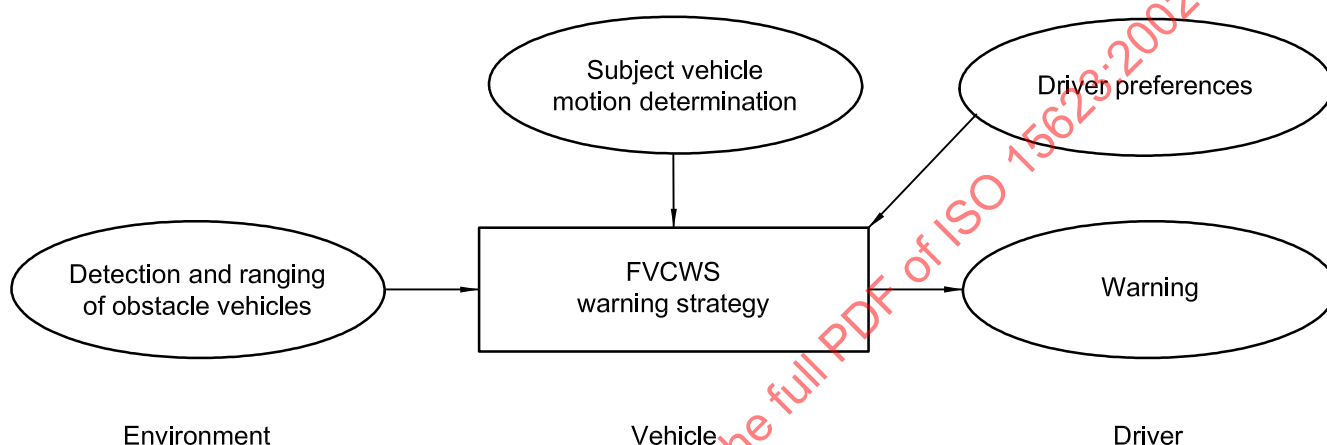
Figure 1 — Functional forward vehicle collision warning system's elements
