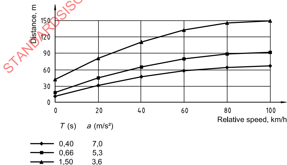
Figure A.6 — Relationship between relative speed and inter-vehicle distance
