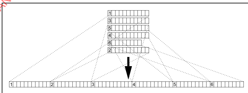
Figure 15 — Defragmentation
