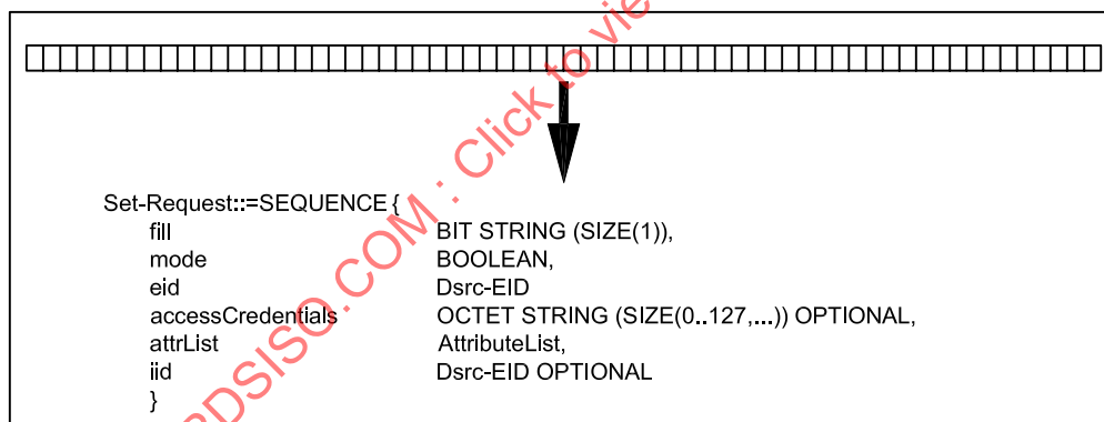
Figure 16 — Decoding
