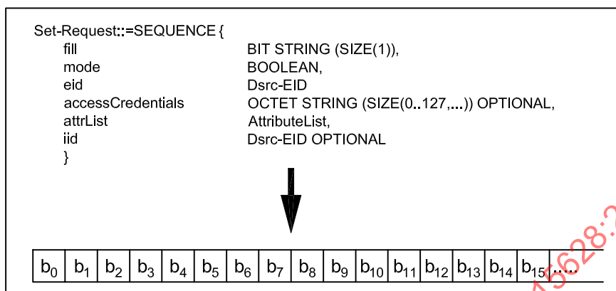
Figure 8 — Encoding
