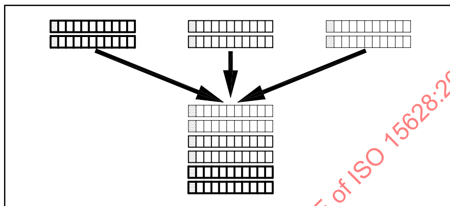
Figure 11 — Multiplexing
