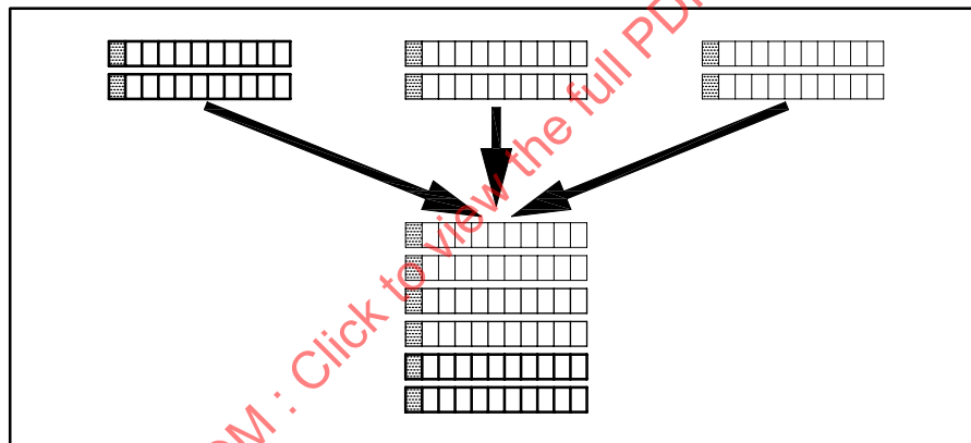
Figure 11 — Multiplexing
