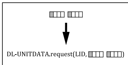
Figure 12 — Concatenation
