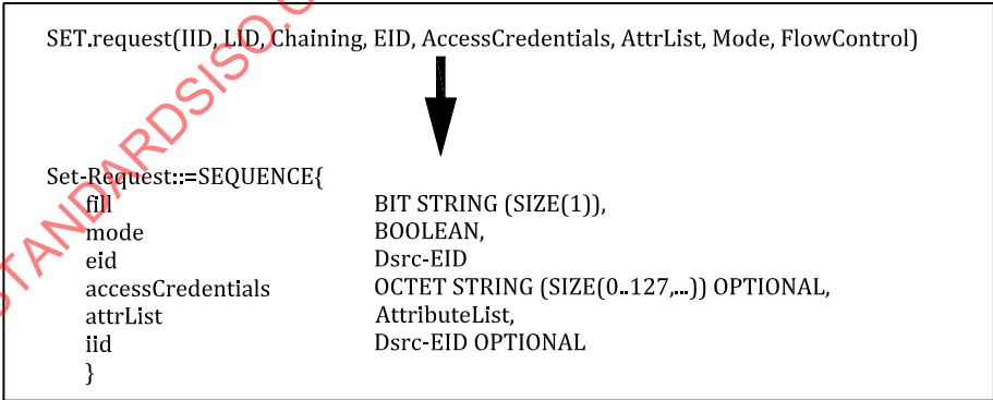
Figure 7 — SDU to PDU
