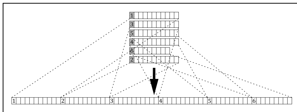
Figure 15 — Defragmentation
