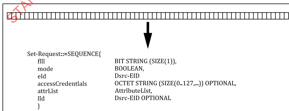
Figure 16 — Decoding
