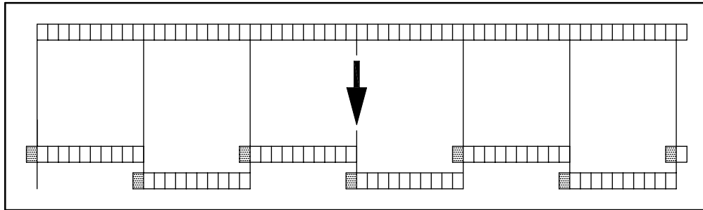
Figure 10 — Fragmentation
