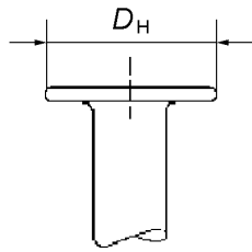
Figure A.14 — Schematic diagram of the nail head diameter measurement
