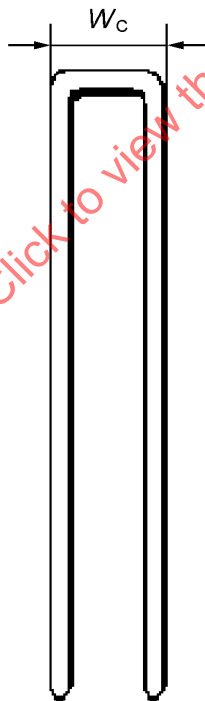
Figure A.18 — Schematic diagram of the staple crown measurement
