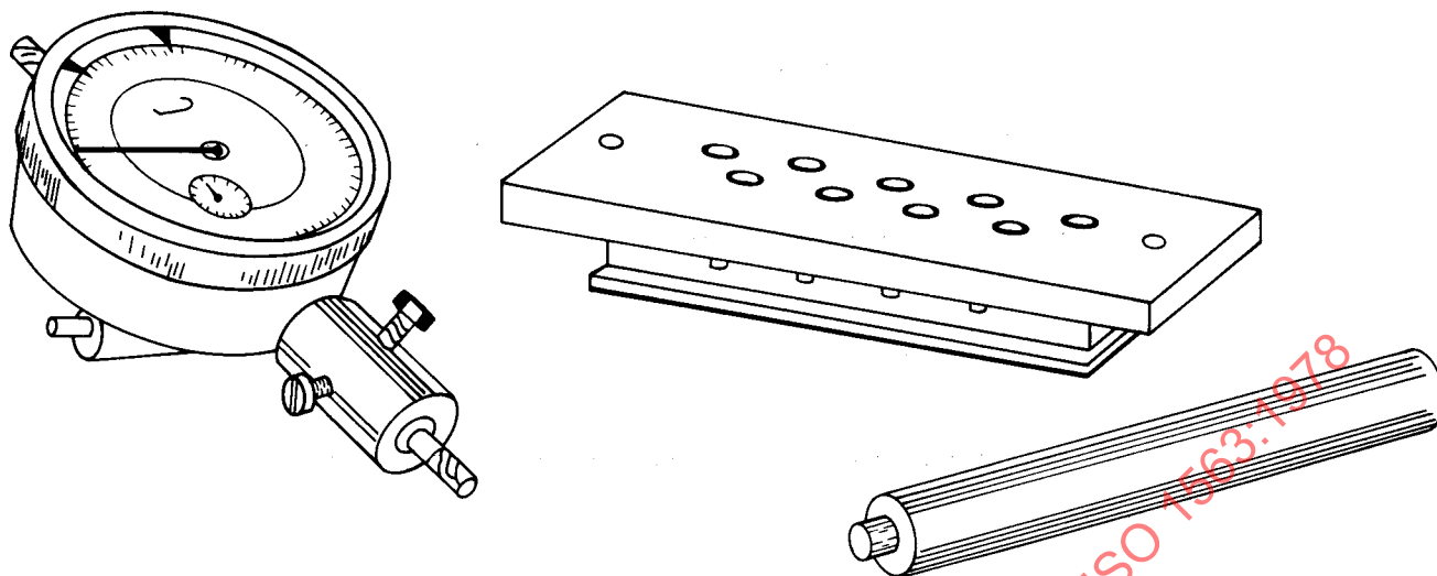
FIGURE 6a) — Apparatus for determination of setting time
