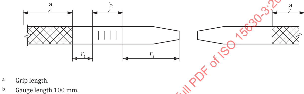
Figure 1 — Measurement of A_{gt} by the manual method
