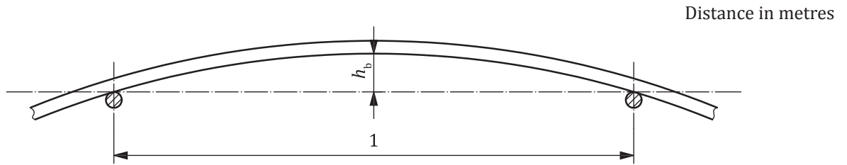
Figure 9 — Measurement of bow height
