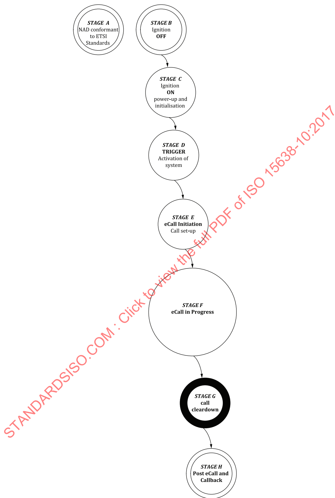
Figure 4 — High level state transition steps of eCall
