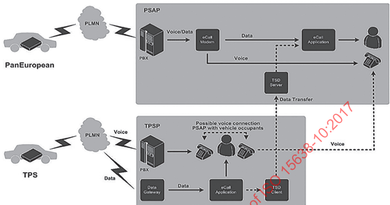
Figure 3 — Use case for end-to-end 'panEuropean eCall' and 'TPS-eCall' systems connected to an 'eCall' enabled PSAP
