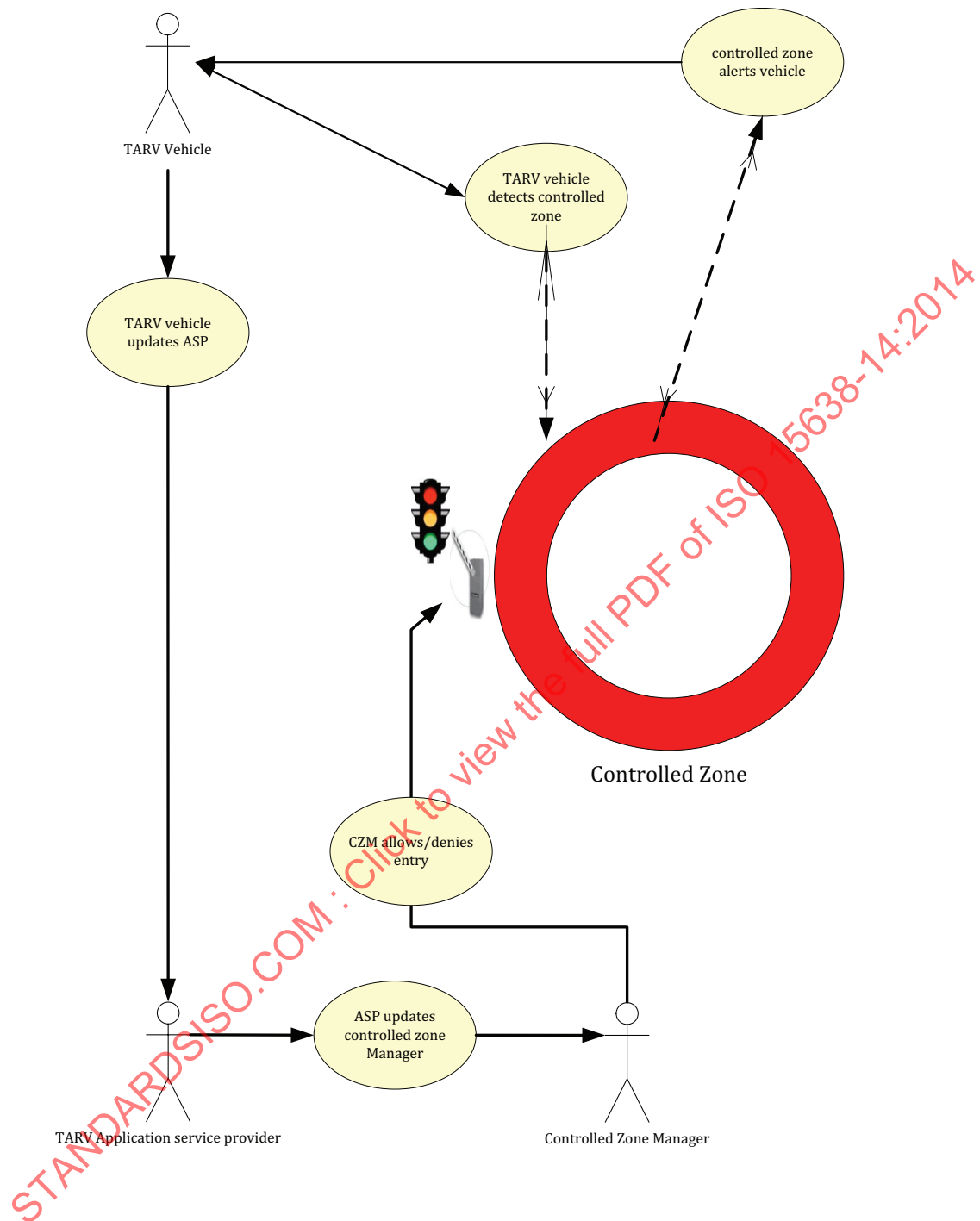
Figure 4 — VAC access control area collaboration diagram
