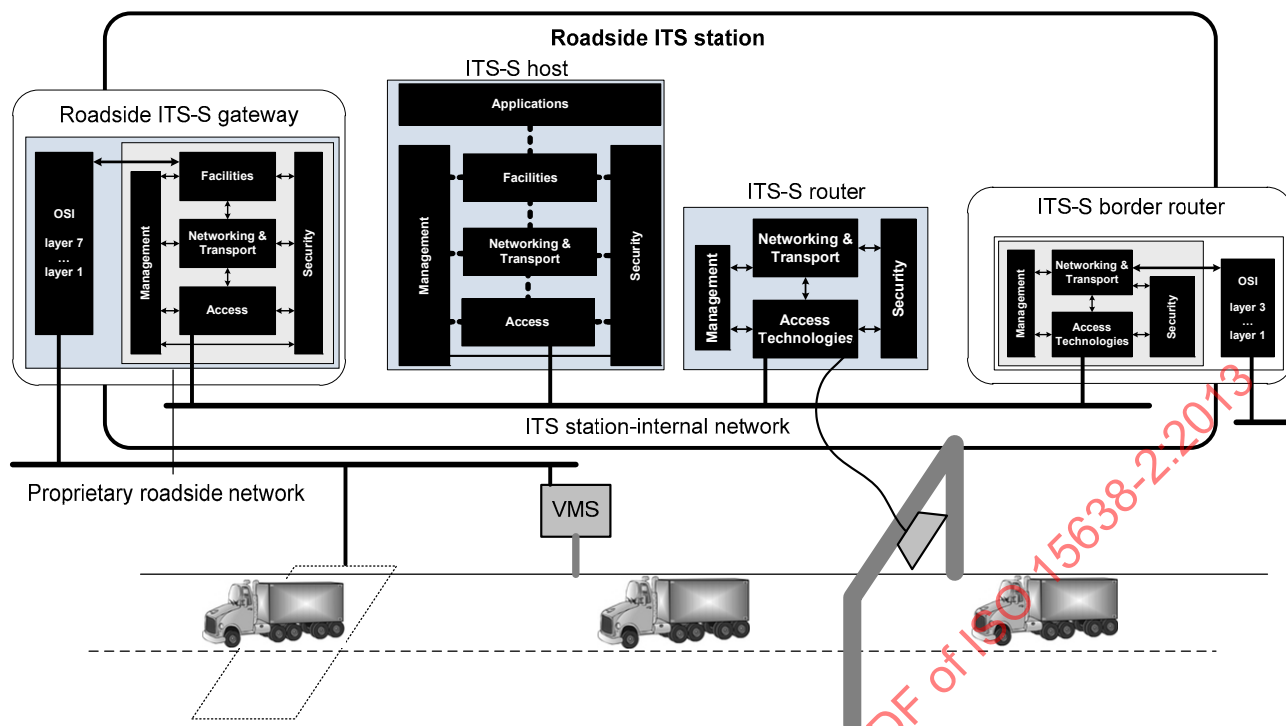
Figure 4 — Roadside ITS subsystem (source ISO 21217)
