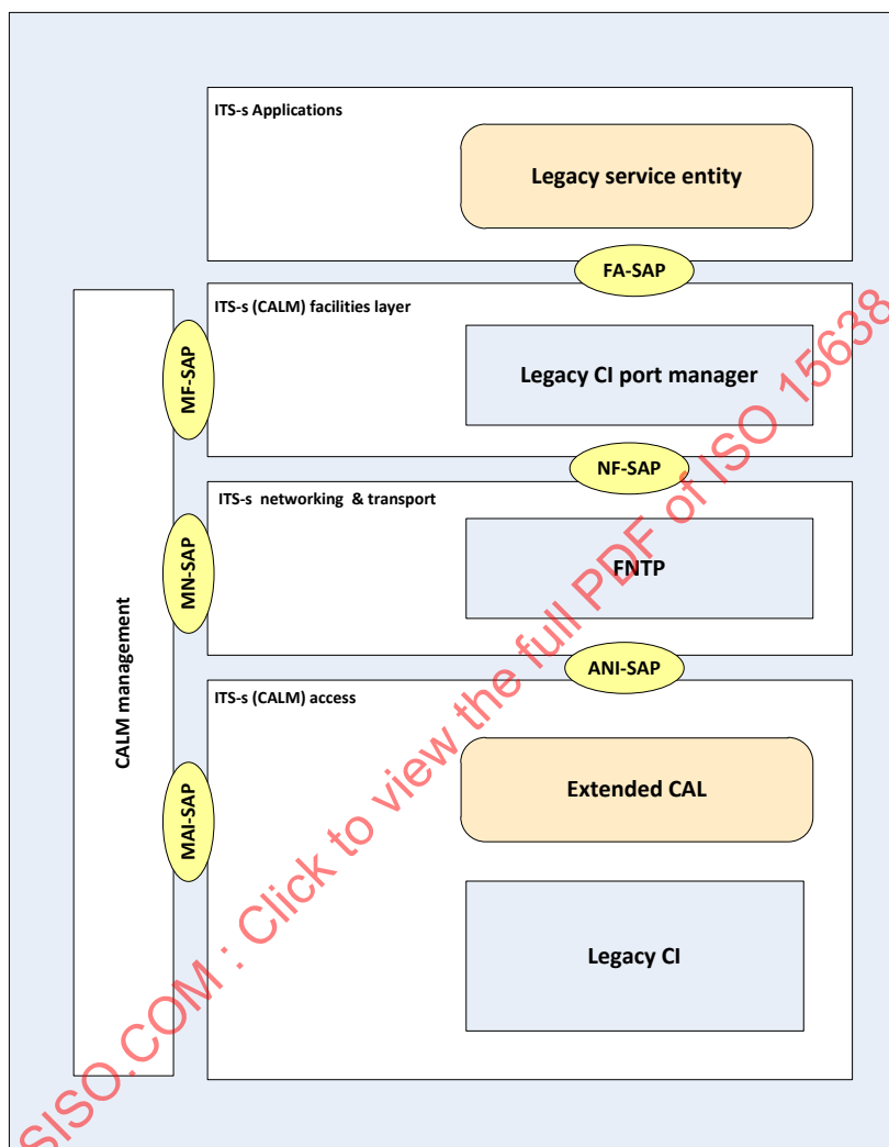
Figure 19 — Legacy communication interfaces (Source: ISO 29281-3 adapted)
