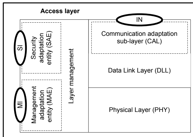
Figure 10 — Elements of access layer (source ISO 21217)
