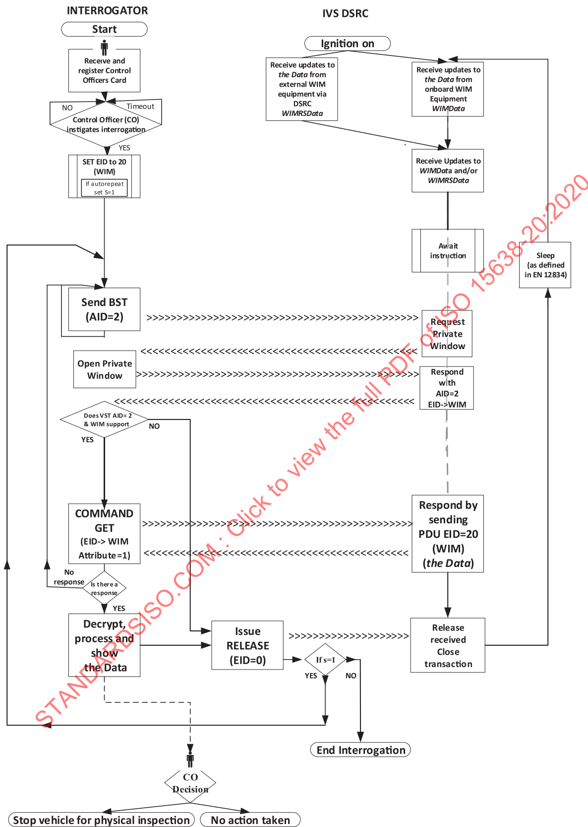
Figure B.5 — WIM over 5,8 GHz DSRC process flow
