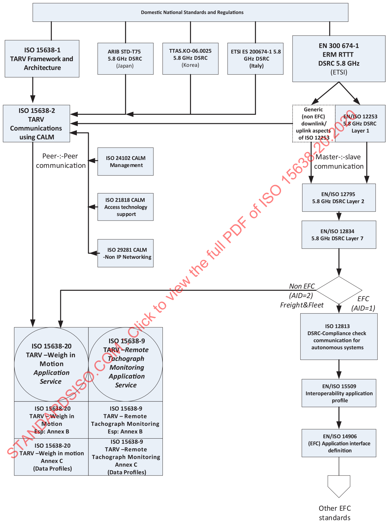
Figure B.3 — Relation and references between ISO 15638-20, CALM Communications and 5,8 GHz DSRC base standards
