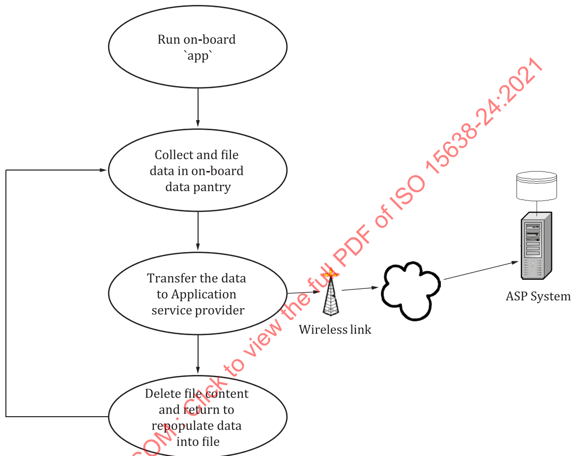
Figure 7 — TARV Regulated application service on-board procedure
