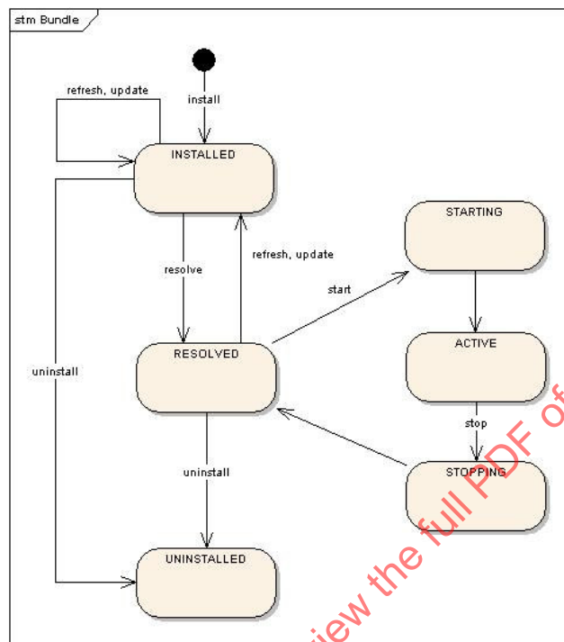
Figure B.6 — CVIS Figure 21: Lifecycle states of JAVA OSGi™ bundles
