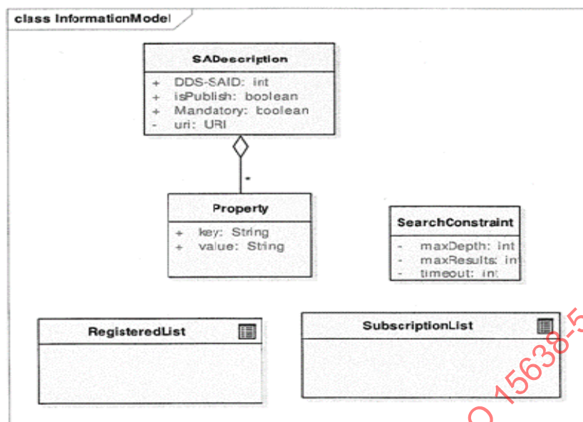
Figure B.8 — CVIS Figure 23: DDS information model
