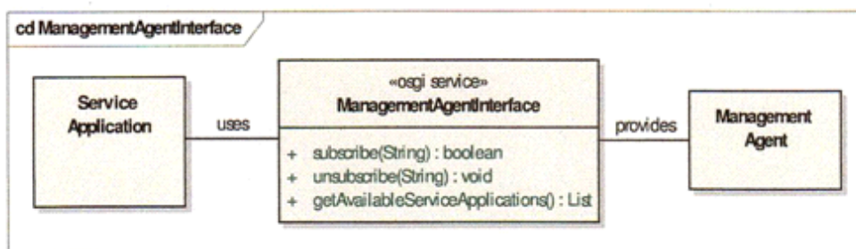
Figure B.4 — CVIS Figure 19: Provisioning API of the CVIS host
