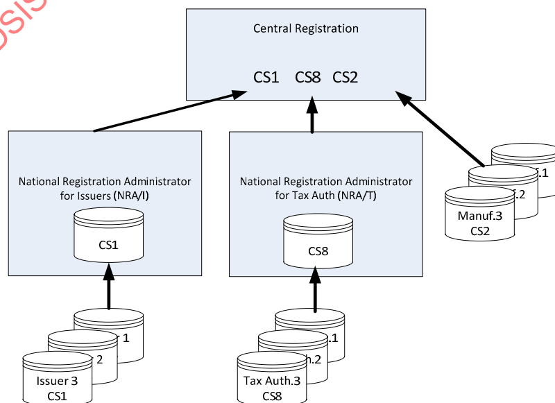
Figure A.1 — Layout of the registration hierarchy
