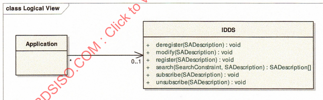
Figure B.7 — CVIS Figure 22: The DDS API
