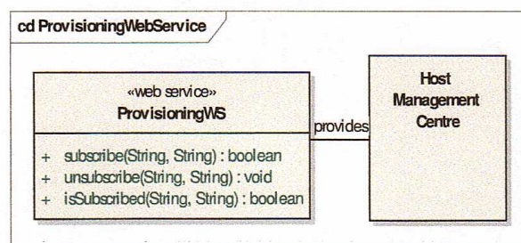
Figure B.3 — CVIS Figure 18 – Provisioning API
