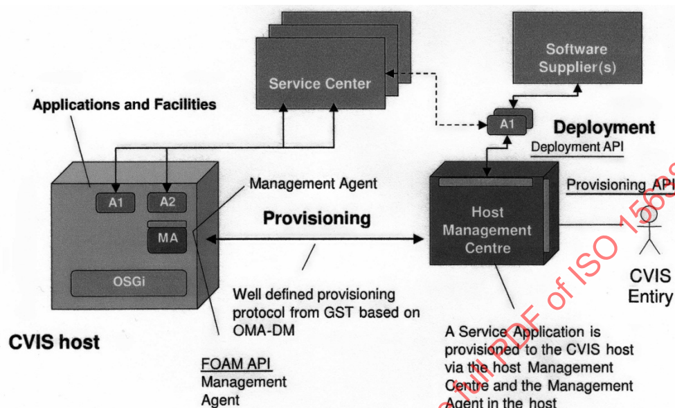
Figure B.1 — CVIS Fig 16 System overview for deployment and provisioning
