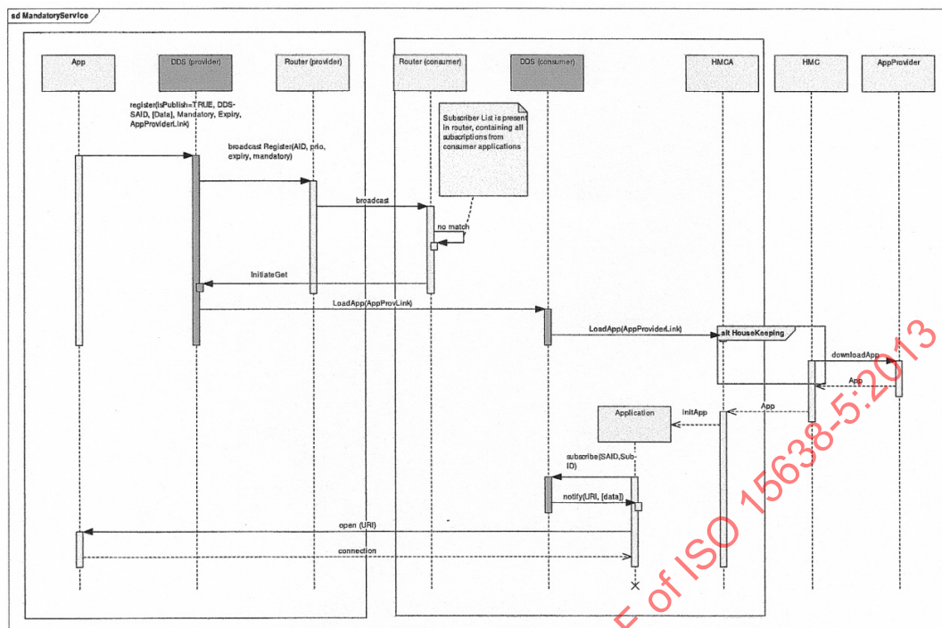
Figure B.12 — CVIS Figure 27: Mandatory service
