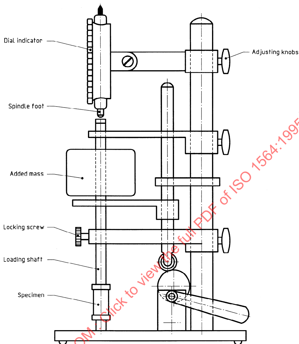
Figure 5 — Apparatus for determining strain in compression
