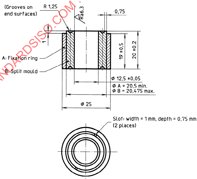
Figure 3 — Split mould for forming specimens for testing properties in compression
