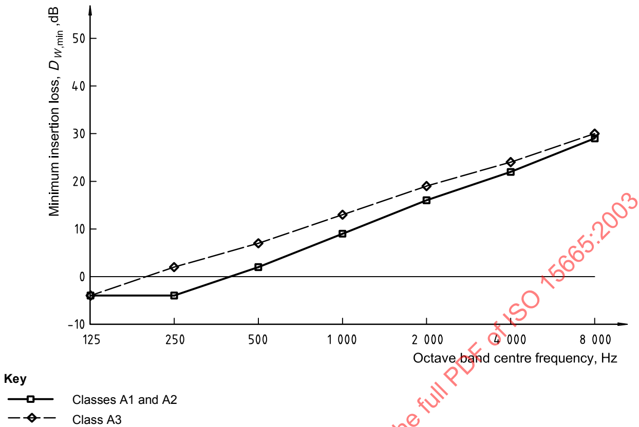
Figure 1 — Minimum insertion loss required for Class A
