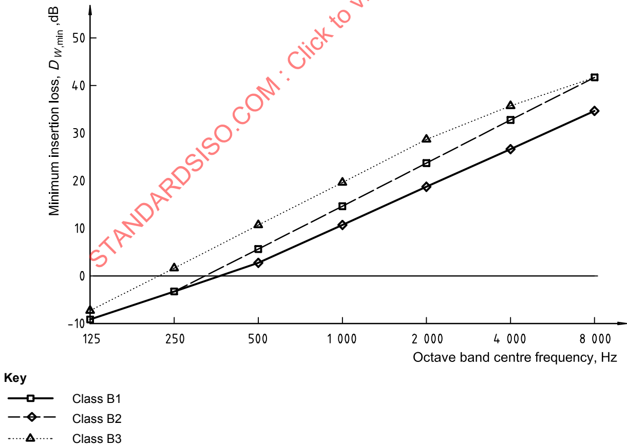
Figure 2 — Minimum insertion loss required for Class B
