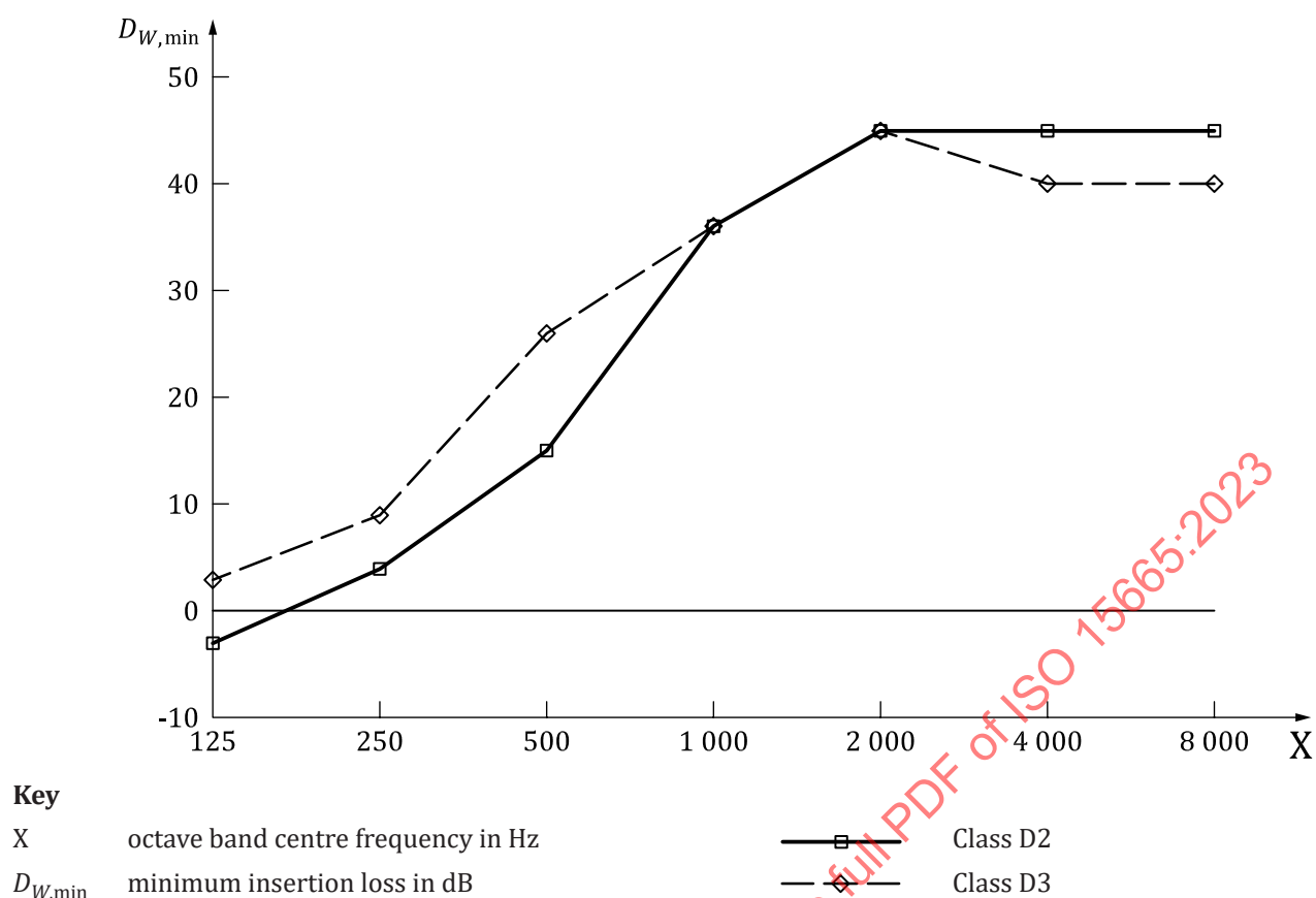
Figure 4 — Minimum insertion loss required for Class D
