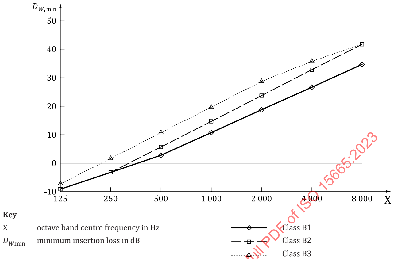
Figure 2 — Minimum insertion loss required for Class B
