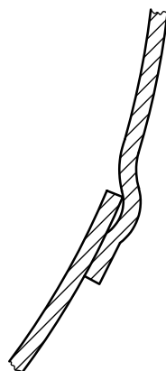
Figure C.2 — Overlap (such that ingress of rain water is prevented)
