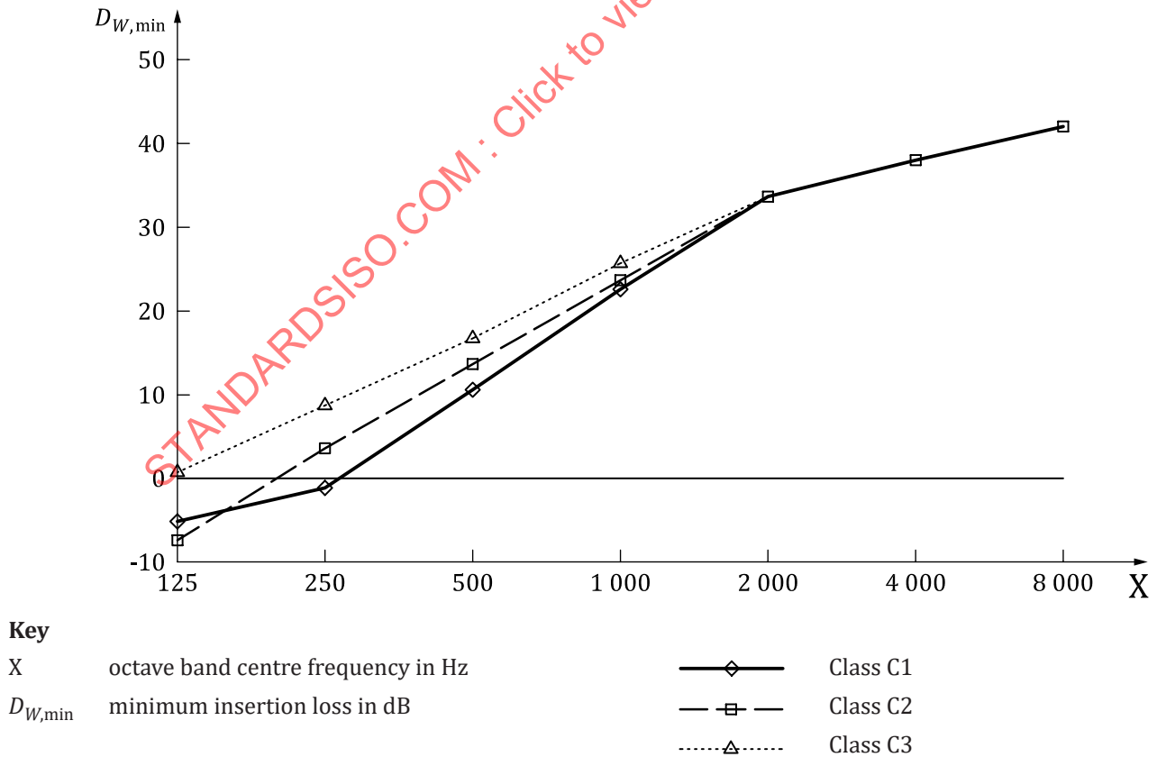
Figure 3 — Minimum insertion loss required for Class C
