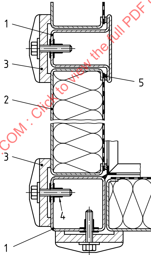
Figure A.3 — Examples of mounting the enclosure wall
