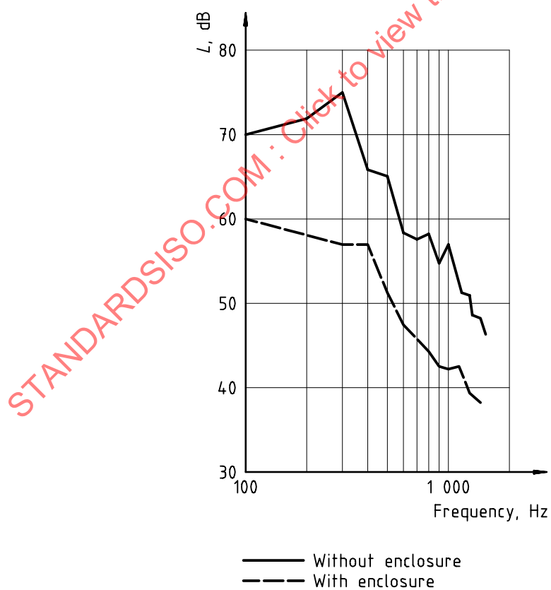
Figure B.3 — Outdoor transformer in enclosure
