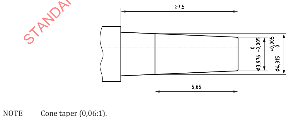
Figure A.5 — Reference steel male conical fitting
