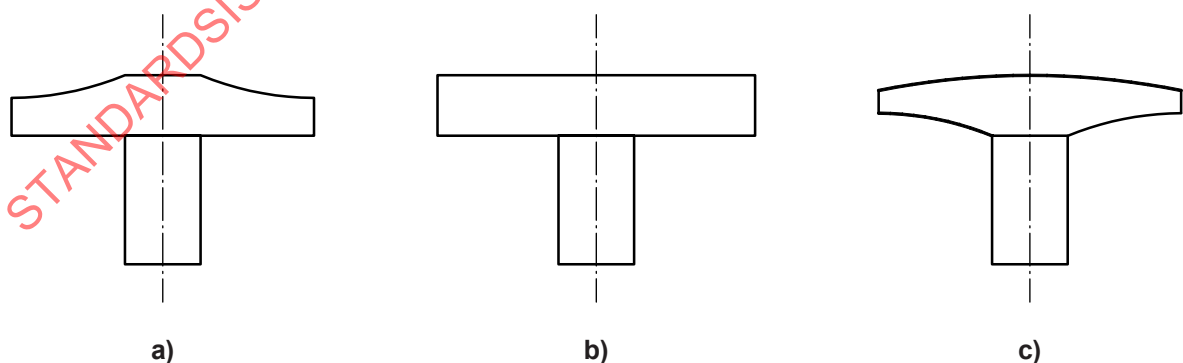
Figure 2 — Examples of head thickness variation
