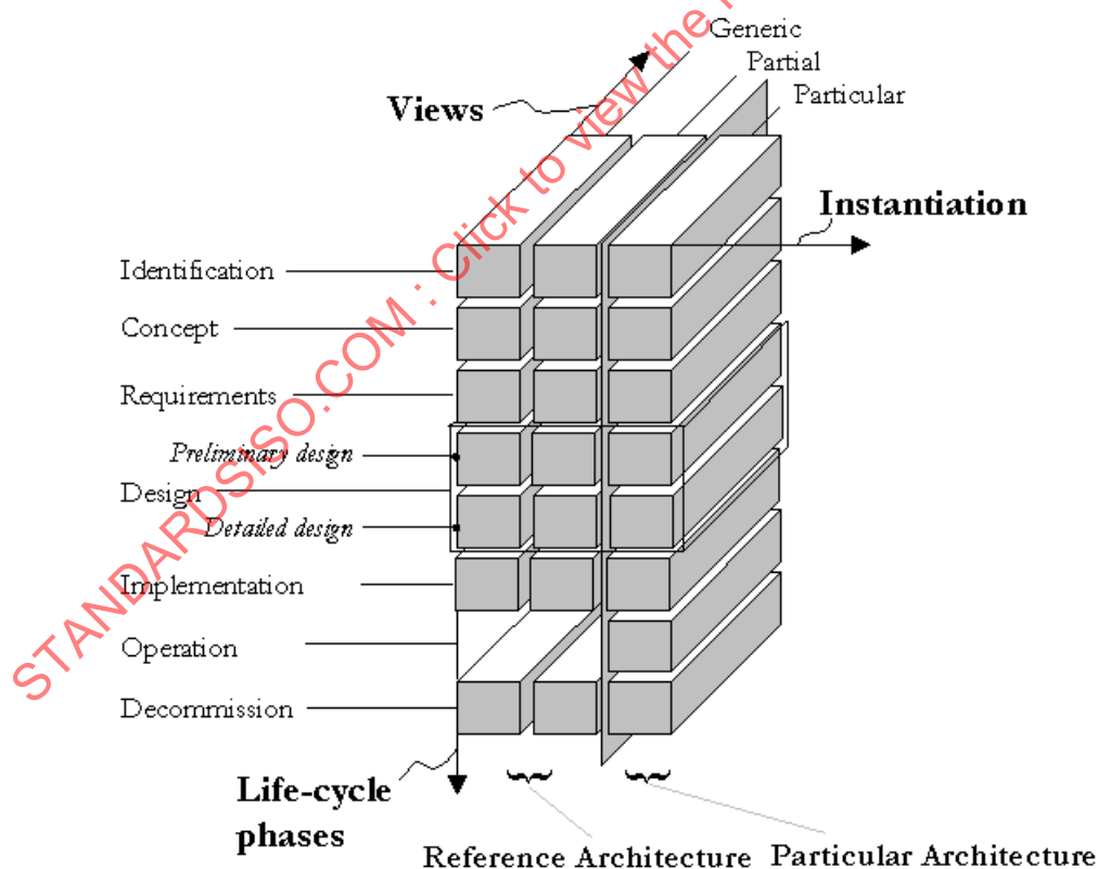
Figure A.8 – The GERA modelling framework
