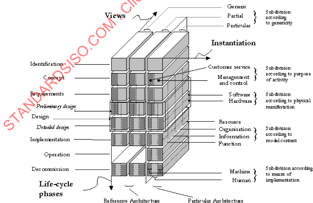
Figure A.10 – GERA modelling framework with modelling views
