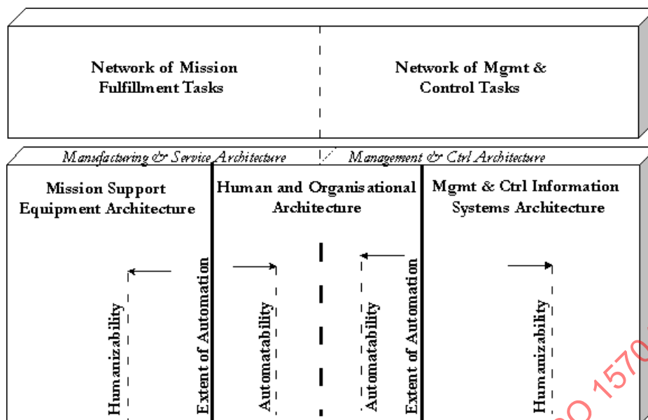
Figure A.11 – Introduction of the concepts of Automatability, Humanizability and Extent-of-Automation lines to define the three implementation architectures
