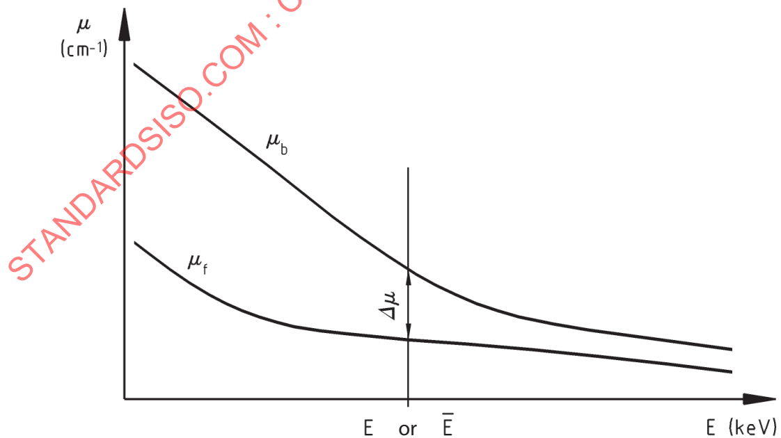
Figure 2 — \Delta\mu as a function of X-ray energy
