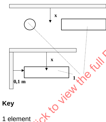
Figure D.1 - Effect on D_{ne} of nearness of reflecting side walls or ceilings (interior or exterior), relative to position without reflecting side walls; small element near two-plane corner, gap element near two- or three-plane corner
