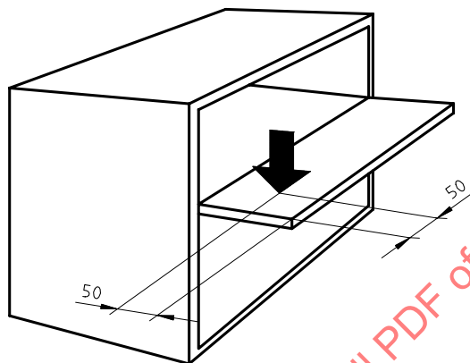
Figure 6 — Strength test for flaps
