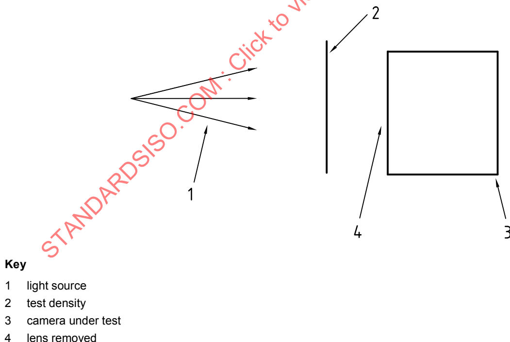
Figure 1 — Illumination for cameras with removable lenses
