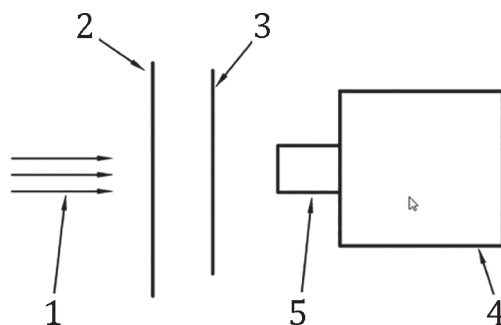
a) Test arrangement using a transmissive test chart
