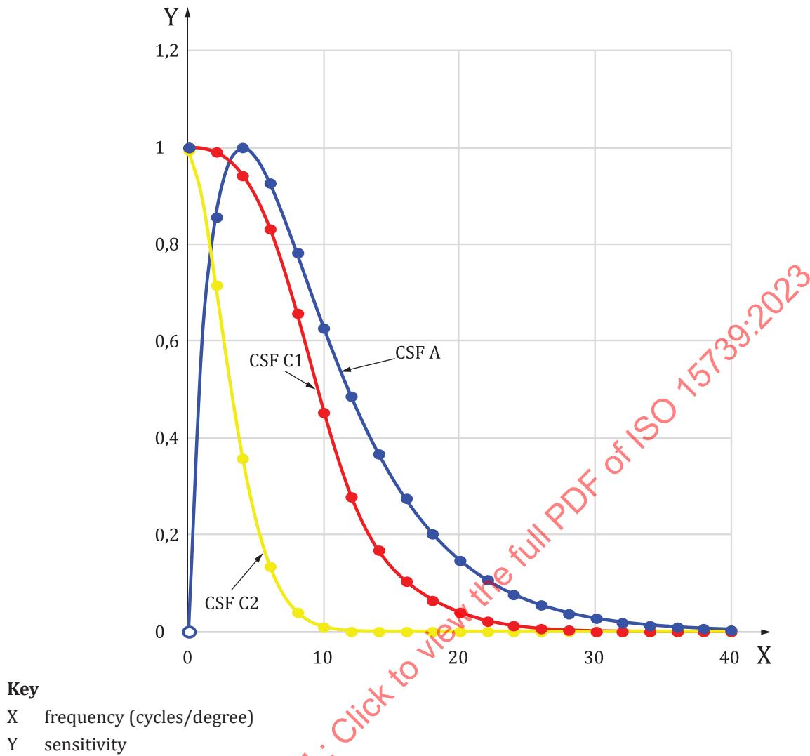
Figure B.2 — Contrast sensitivity functions of the human eye used in ISO 15739
