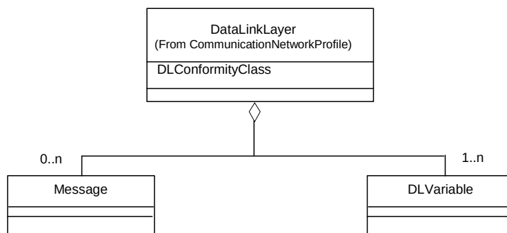
Figure 18 — WorldFIP communication network profile – Data Link layer
