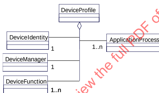
Figure 9 — WorldFIP device profile class diagram
