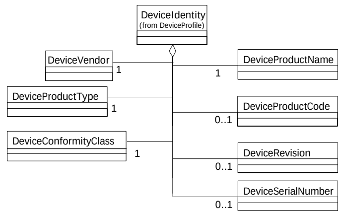
Figure 10 — WorldFIP DeviceIdentity class diagram
