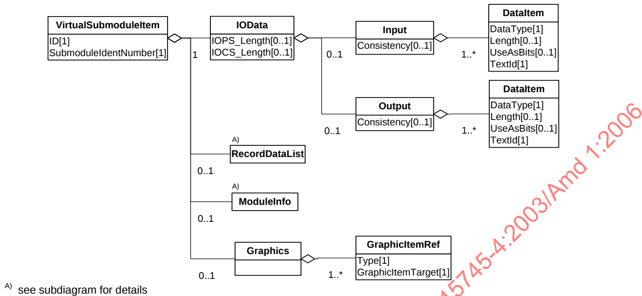
Figure 16 — PROFINET VirtualSubmoduleItem class diagram
