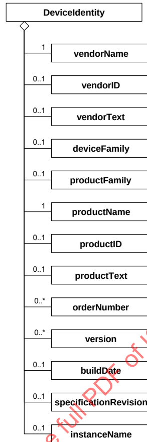
Figure 27 — EtherCAT DeviceIdentity class diagram
