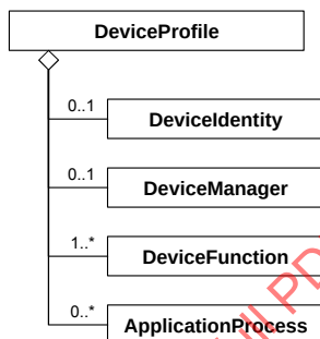
Figure 26 — EtherCAT device profile class diagram
