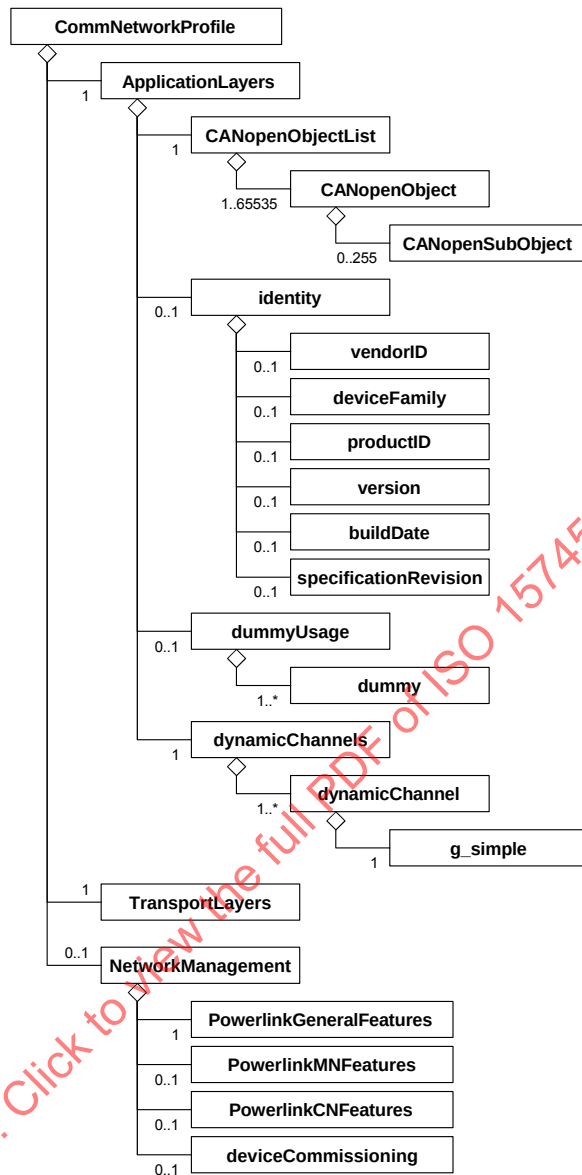
Figure 37 — ETHERNET Powerlink communication network profile class diagram
