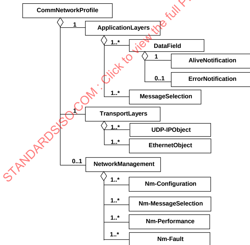
Figure 2 — ADS-net communication network profile class diagram
