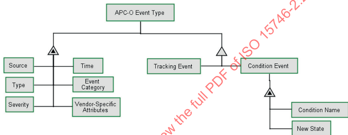
Figure 7 — APC-OEvent Type Information Model
