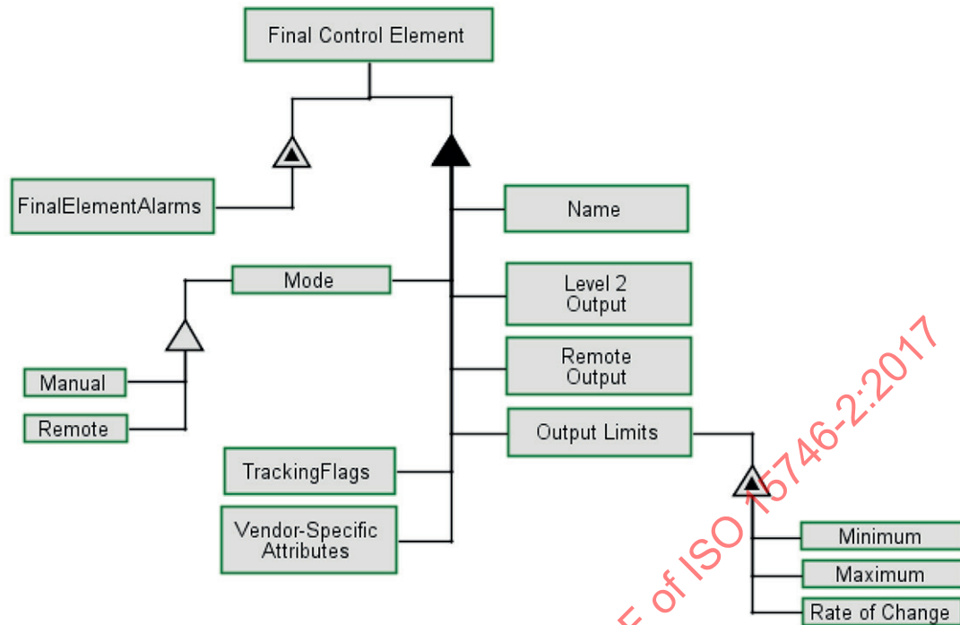
Figure 11 — FinalControlElement Information Model
