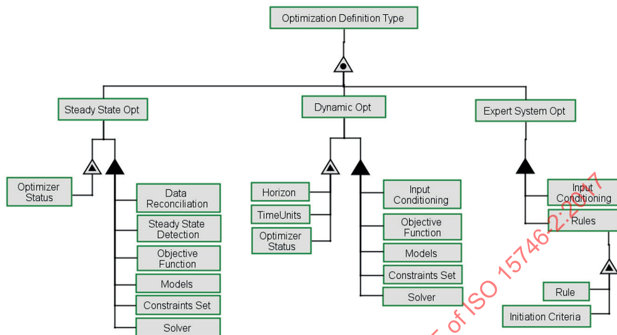
Figure 21 — Example Optimization Definition Types
