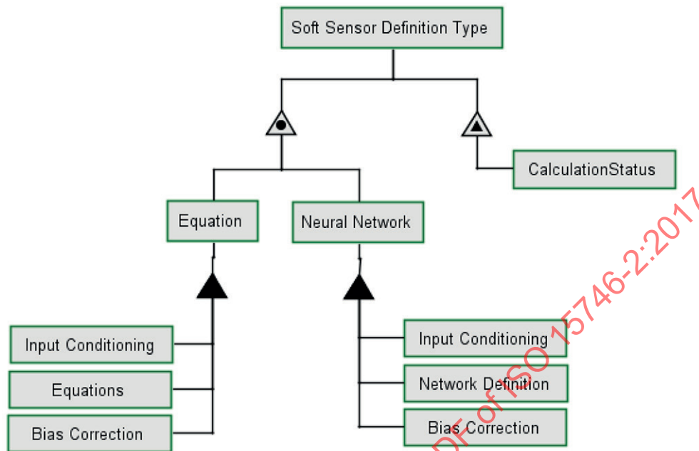
Figure 20 — Example SoftSensorDefinition Types
