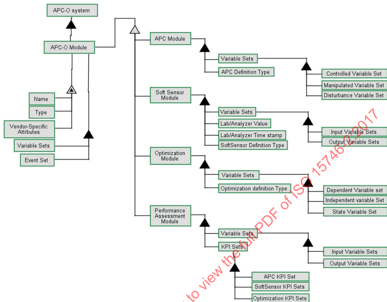
Figure 6 — APC-O Information Model
