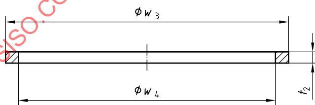
Figure A.10 — Elastomer plug washer
