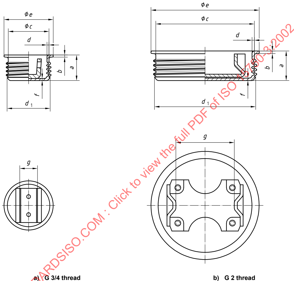
Figure C.4 — Steel plug
