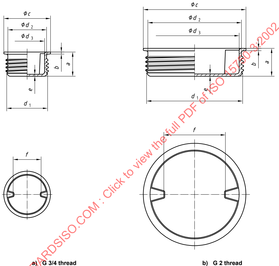
Figure C.3 — Zinc-alloy die cast plug
