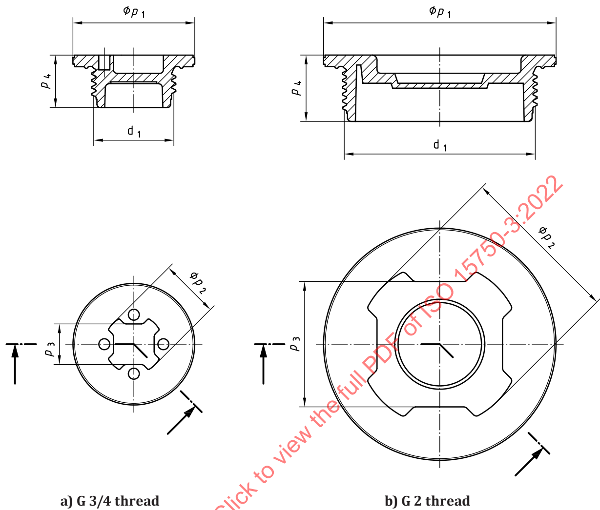
Figure B.6 — Plastics plug
