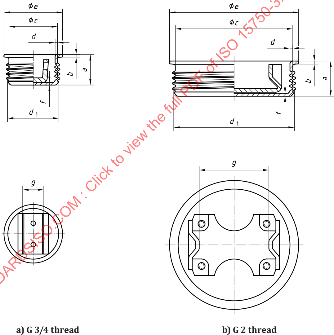
Figure C.3 — Steel plug
