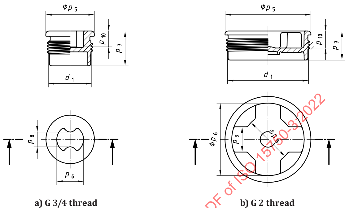
Figure A.9 — Plastics plug
