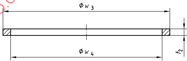
Figure A.8 — Elastomer plug washer
