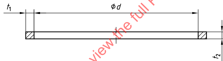
Figure C.5 — Washer for flange
