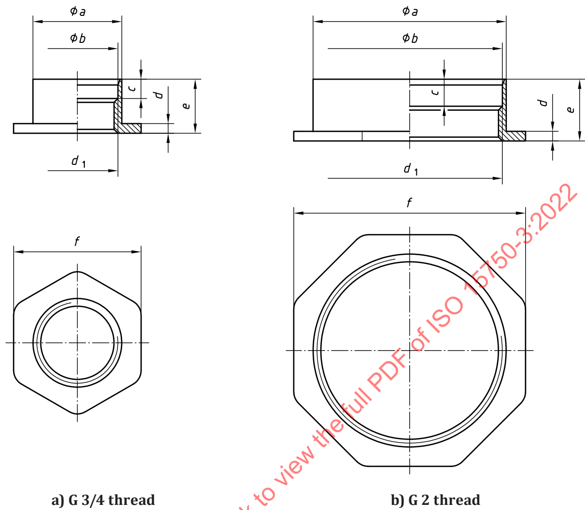
Figure C.2 — Flange
