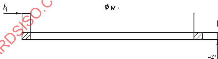
Figure B.7 — Elastomer plug washer
