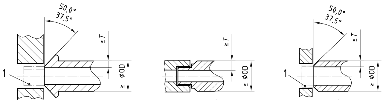
a) Integrally reinforced end for welding
