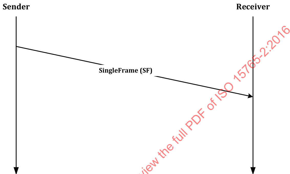
Figure 3 — Example of an unsegmented message
