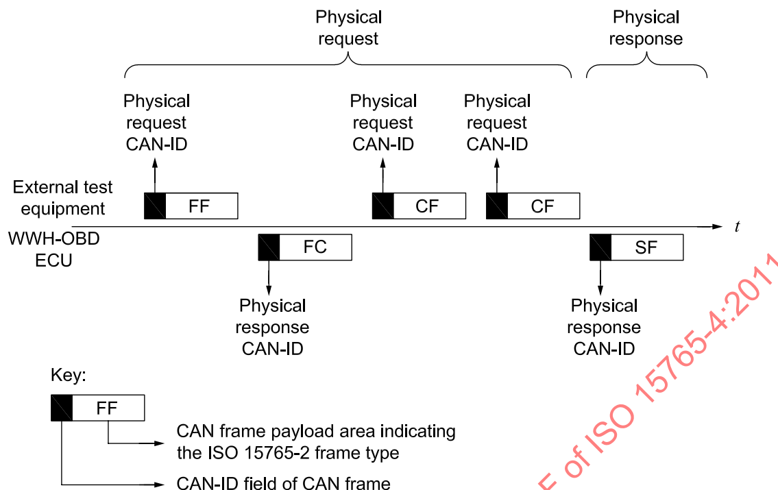
Figure 7 — Physical request CAN identifier usage
