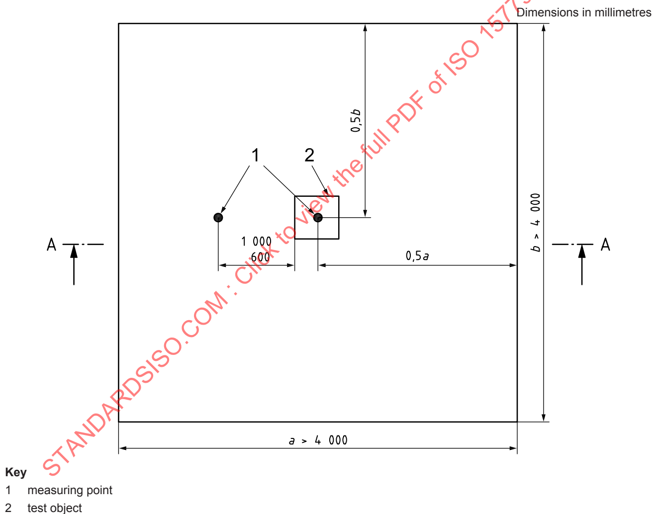
Figure D.5 — Plan view of instrumentation placement for the extinguishing factor test
