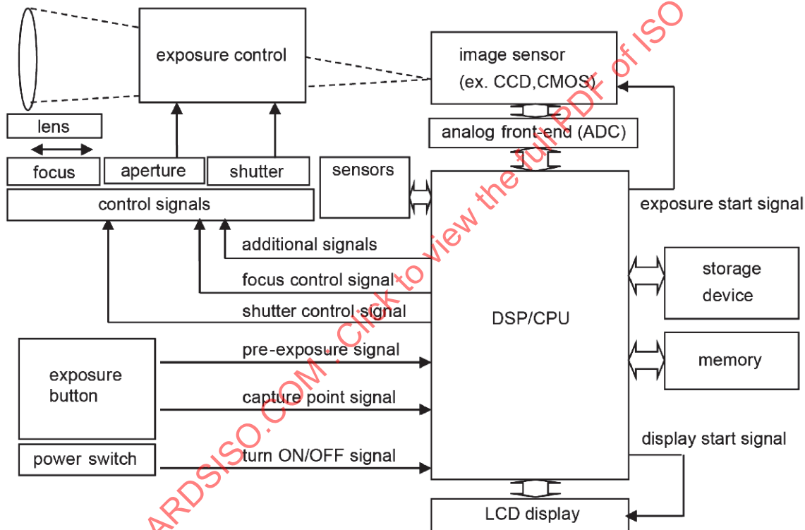
Figure C.1 — Block diagram of a standard digital still camera
