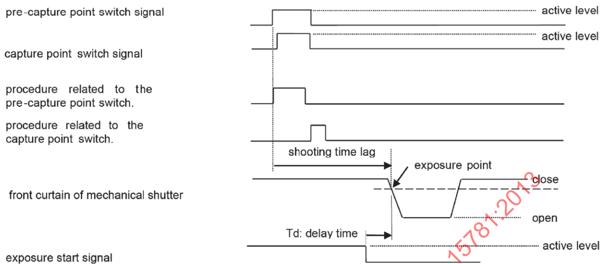
Figure C.4 — Measurement point of shooting time lag (mechanical shutter)
