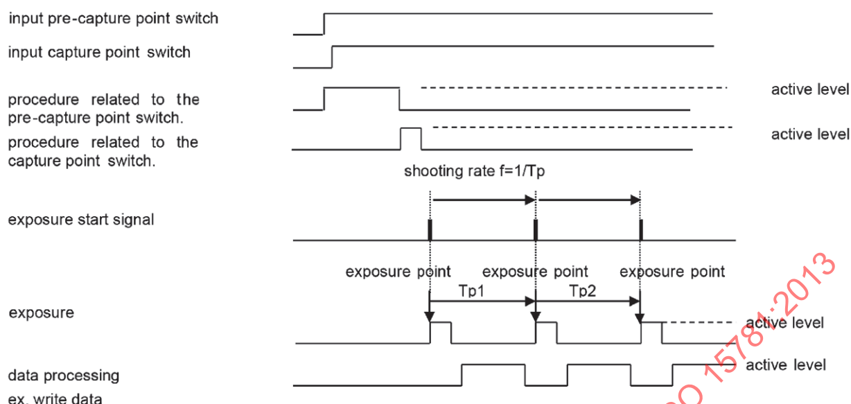
Figure C.3 — Measurement point of shooting rate
