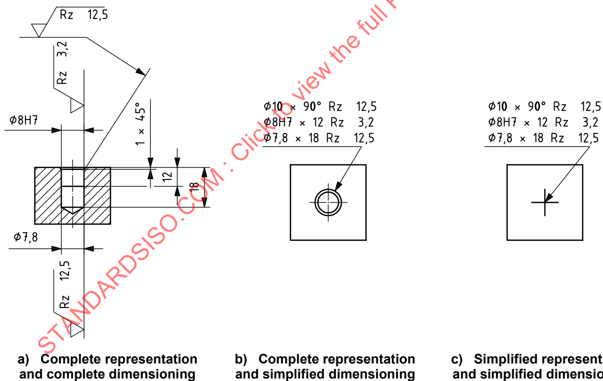
Figure 18 — Complex chamfered hole with surface roughness indications (hole bottom not specified)
