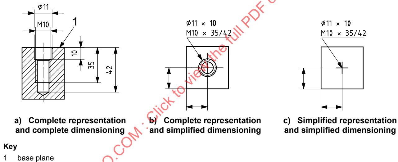
Figure 15 — Complex threaded countersunk hole with indication of thread length and cored hole depth (hole bottom not specified)
