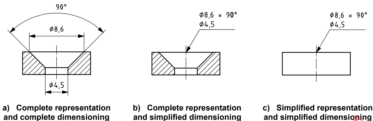
Figure 11 — Chamfer
