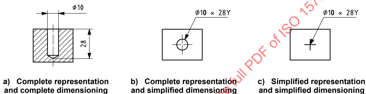
Figure 8 — Hole with dimension indicated up to bit
