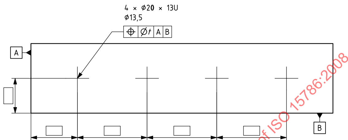
Figure 19 — Simplified representation of group of four holes with counterbore using tolerance frame
