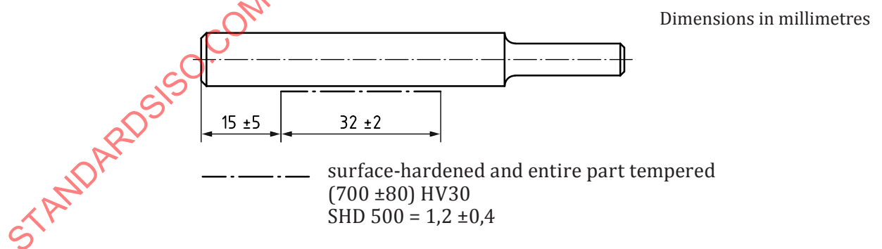
Figure 15 — Marking of a part which is surface-hardened
