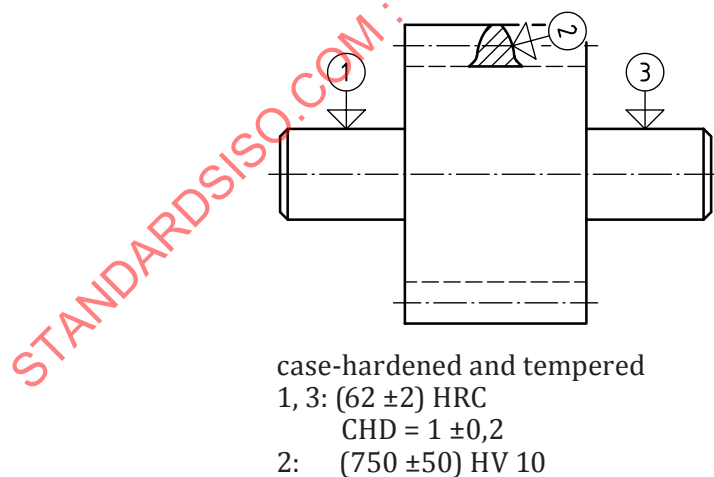
Figure 32 — Marking of a case-hardened and tempered part with different hardnesses and hardness depths
