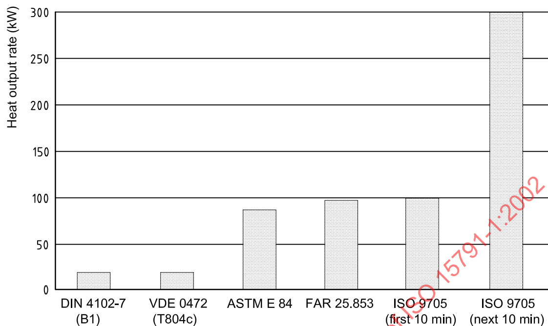
Figure 3 — Power of standardized gas burners
