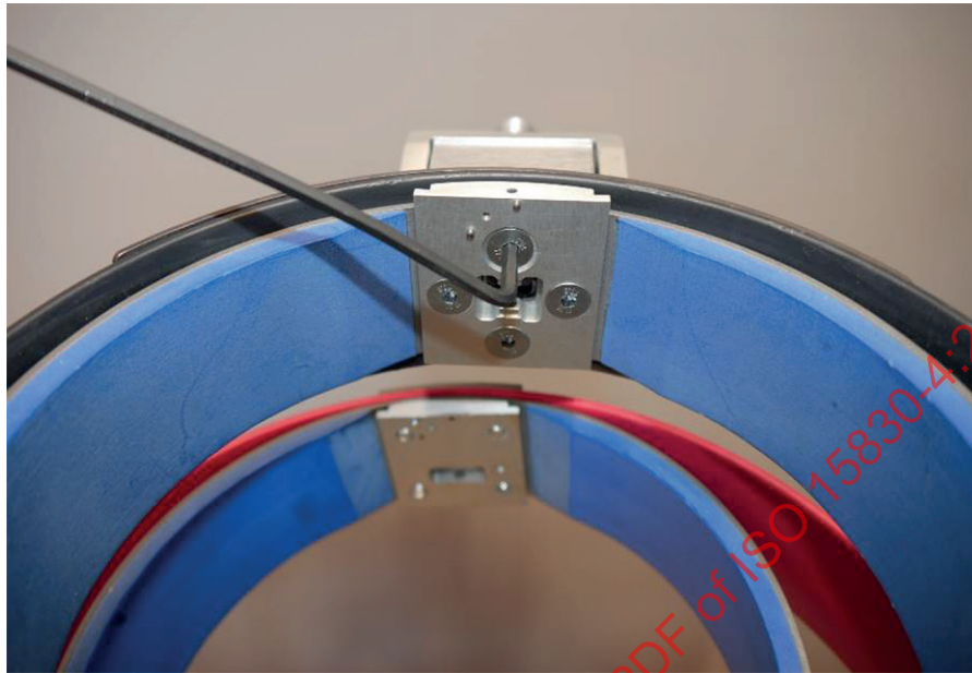
Figure A.19 — Removal of shoulder load cell assembly
