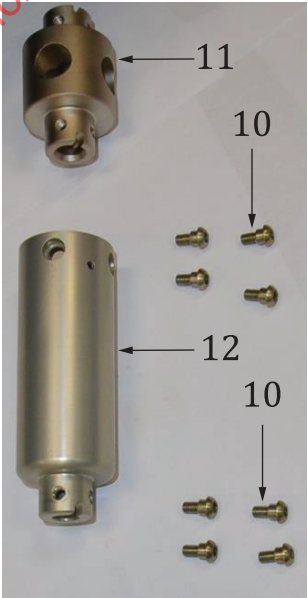
Figure A.54 — Upper leg components
