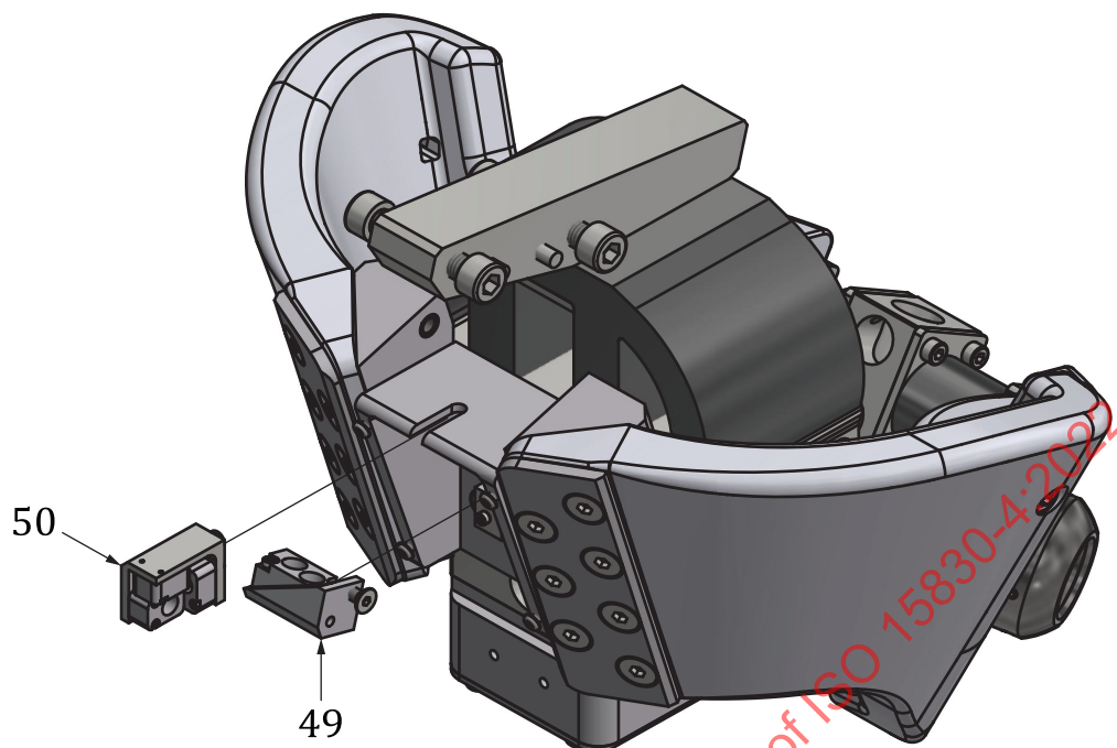
Figure A.33 — WorldSID pelvis components rear view
