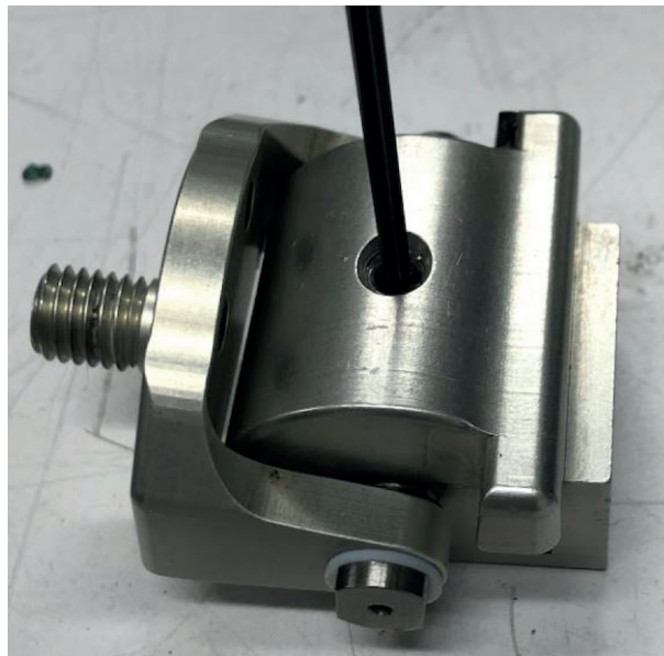
Figure A.21 — Removal of set screw from shoulder load cell structural replacement
