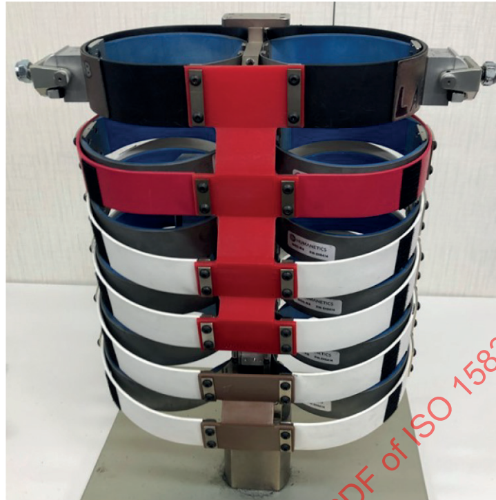
Figure A.23 — Rib colour scheme
