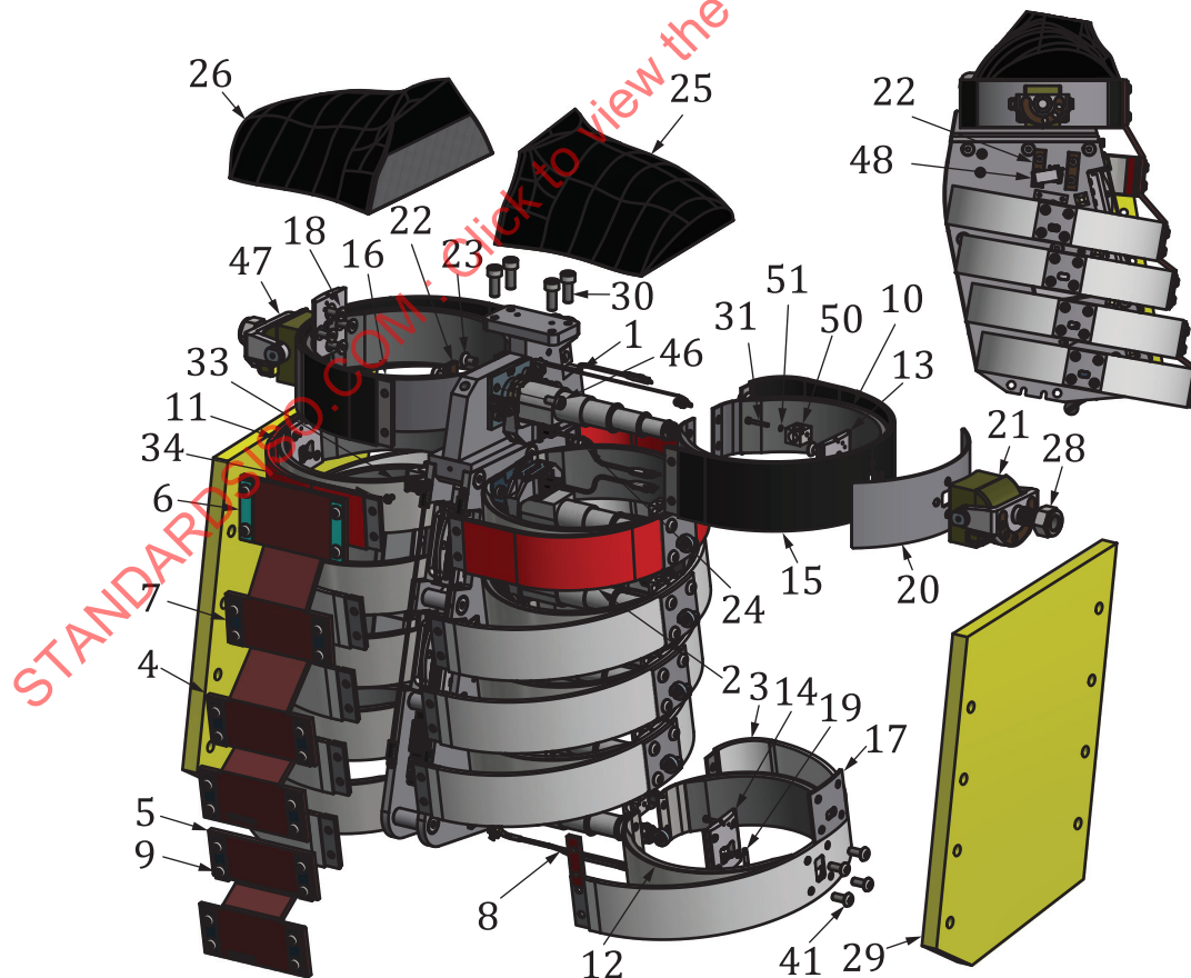
Figure A.15 — WorldSID thorax and abdomen components
