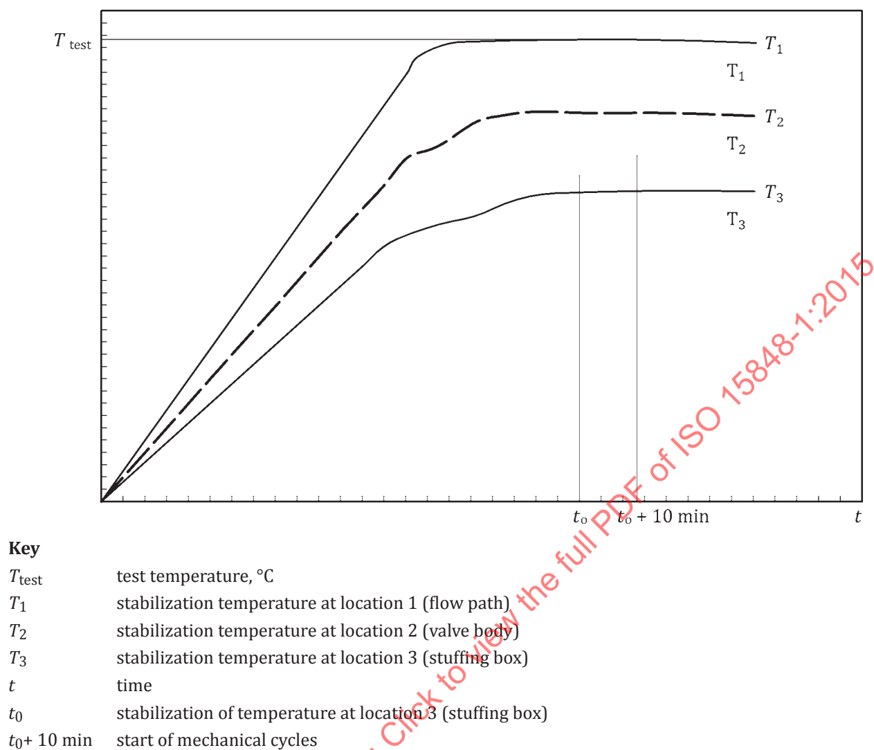
Figure 2 — Stabilization of temperatures (when the valve is internally heated or cooled)
