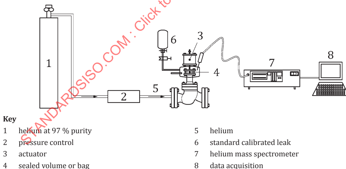
Figure A.7 — Equipment
