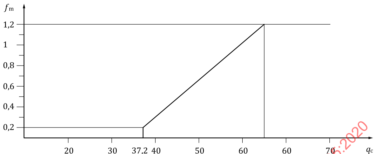
Figure 1 — Engine factor, f_m , as a function of corrected fuel delivery parameter, q_c
