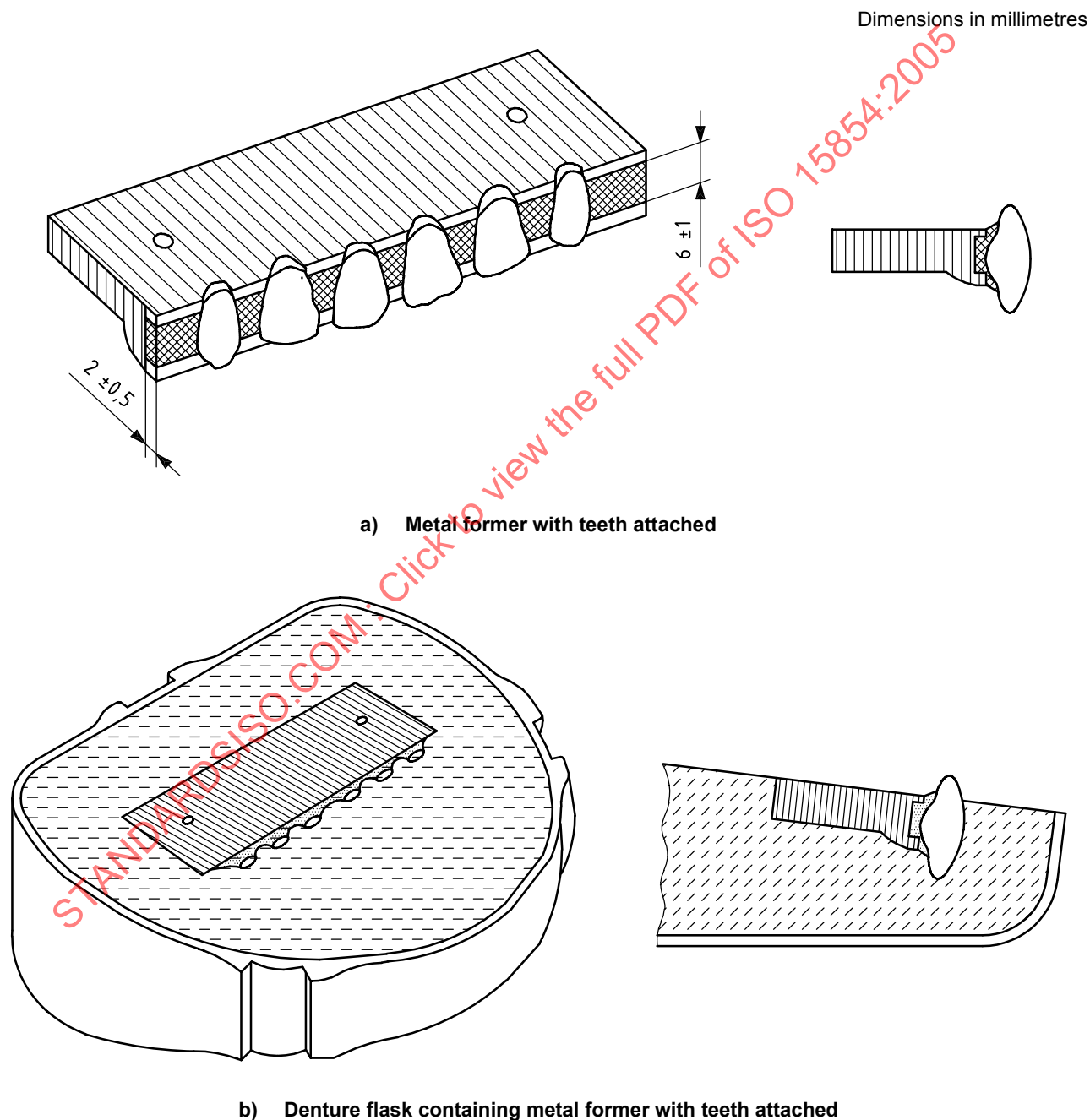
Figure 4 — Apparatus for test for residue on artificial teeth and behaviour of colouring material
