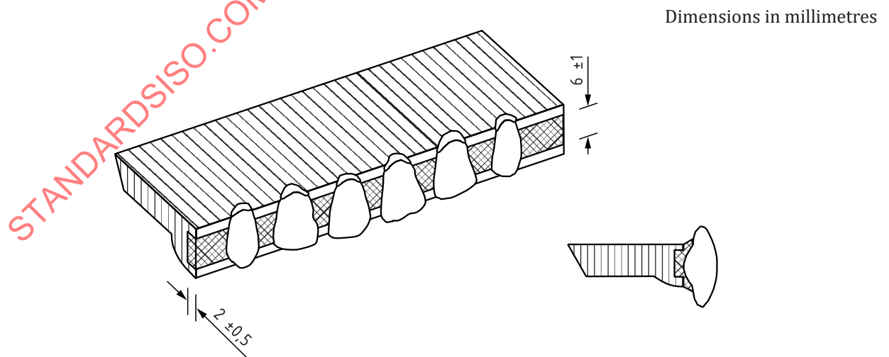
a) Example of a suitable metal former with teeth attached
