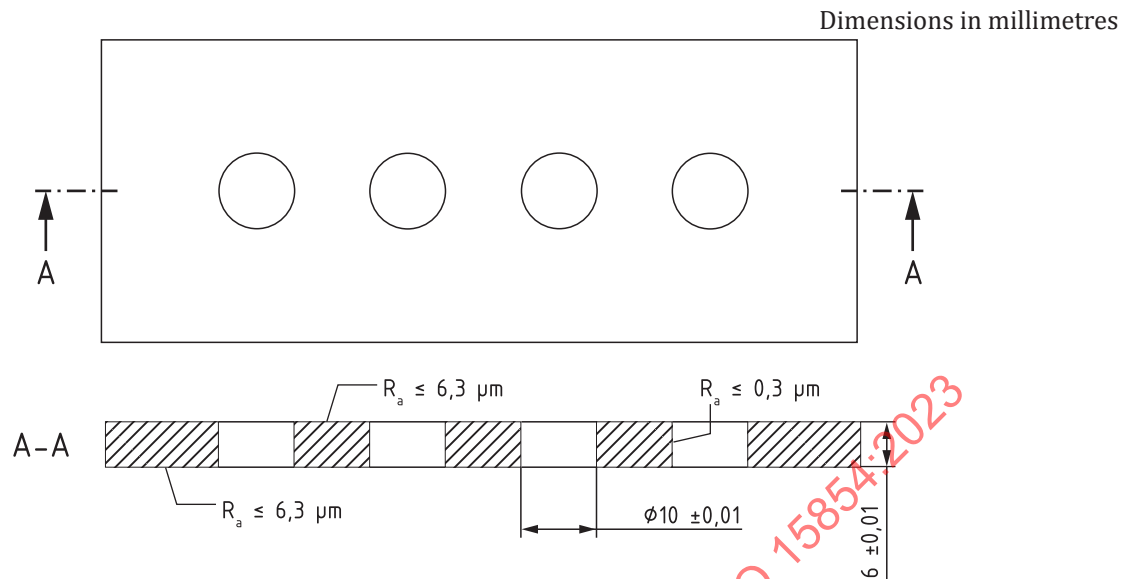
Figure 3 — Example of a suitable mould for preparing flow test pieces
