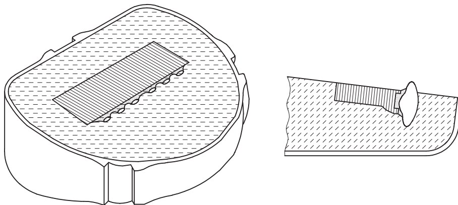
b) Lower portion of denture flask containing invested metal former with teeth attached
