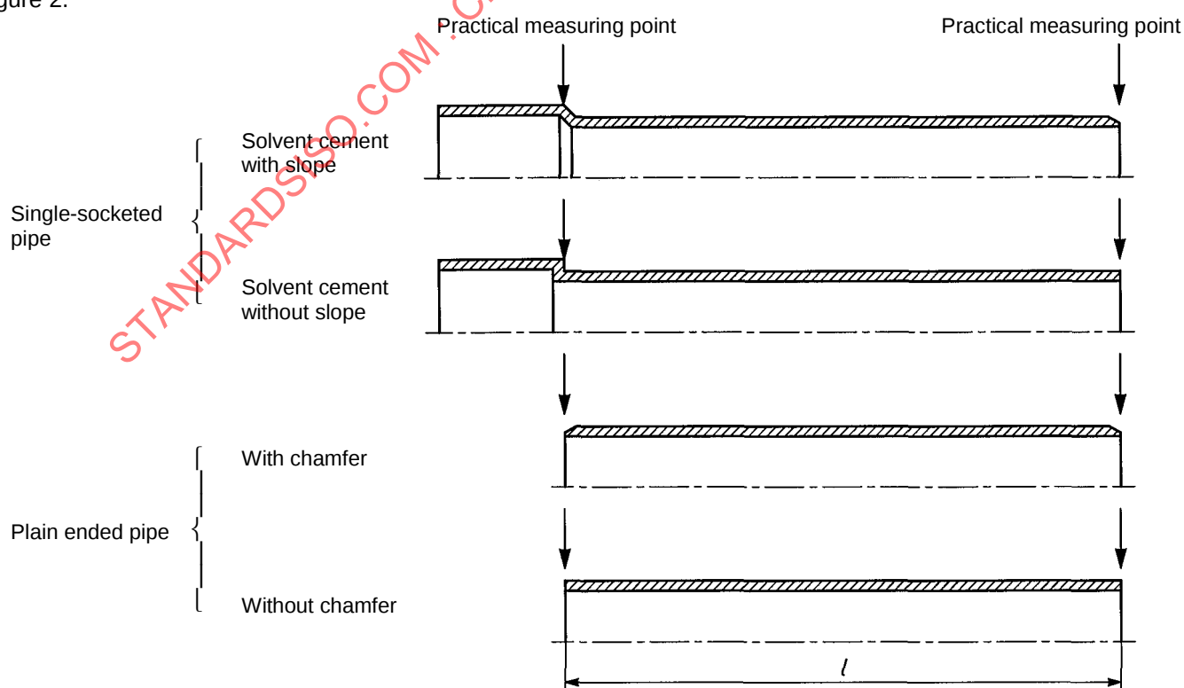
Figure 2 — Effective length of pipes
