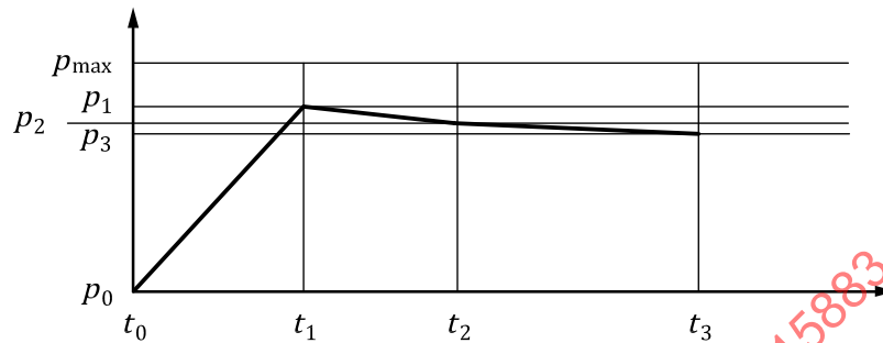
Figure 1 — Pressure versus time graph for leak test
