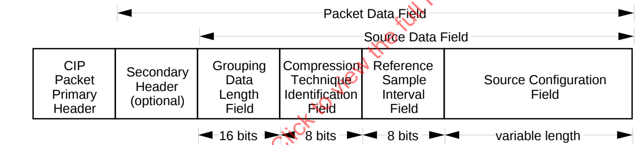
Figure 6-1: Compression Identification Packet Structure
