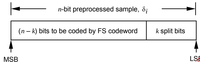
Figure 3-2: Split-Sample Format
